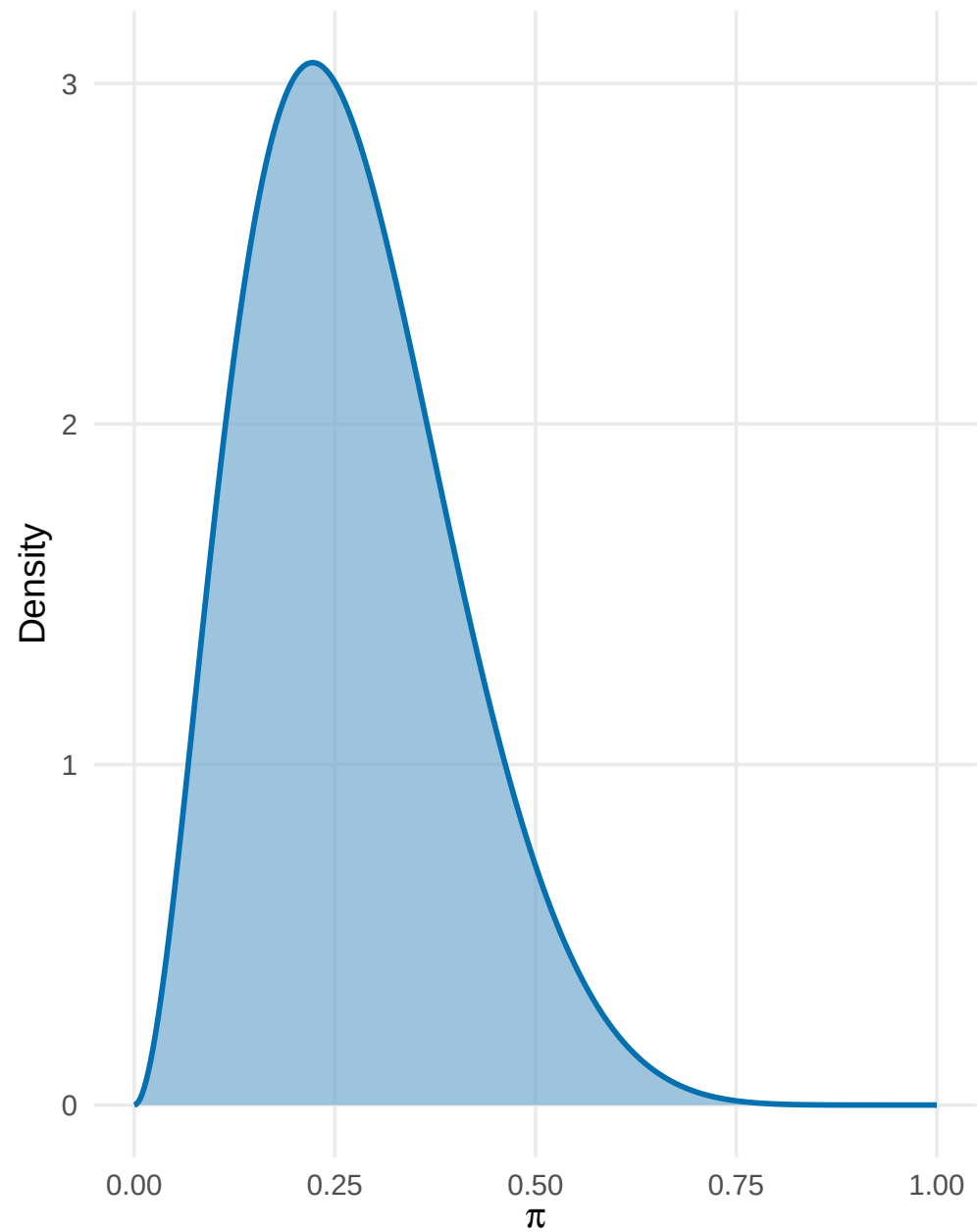
Beta(3, 8) prior on edge probability
